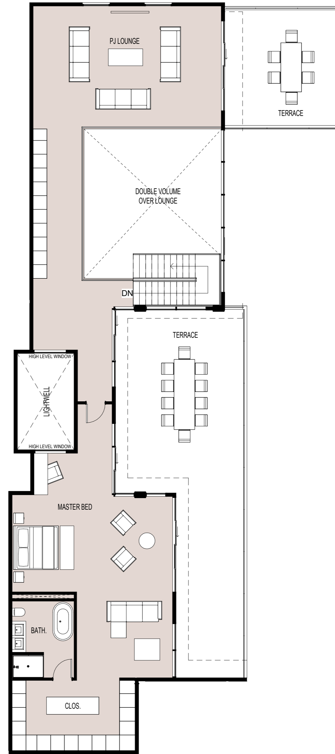
PENTHOUSE 1 UPPER SCALE: 1 : 100 UPPER LEVEL
